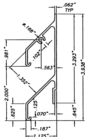
(I) HALF SHUTTER BLADE SCALE: 1/2" = 1"
