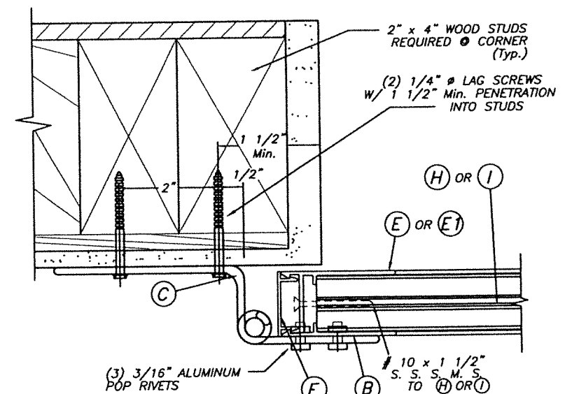
DETAIL 4A (PLAN)
