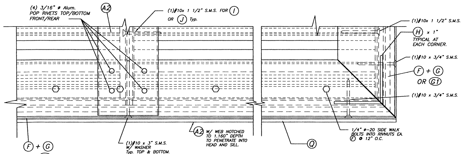
DETAIL 1
