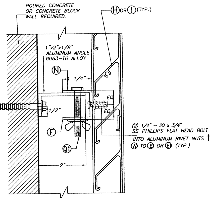
ELEVATION Y-Y
