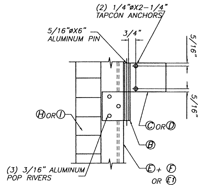
ALTERNATE DETAIL 3
