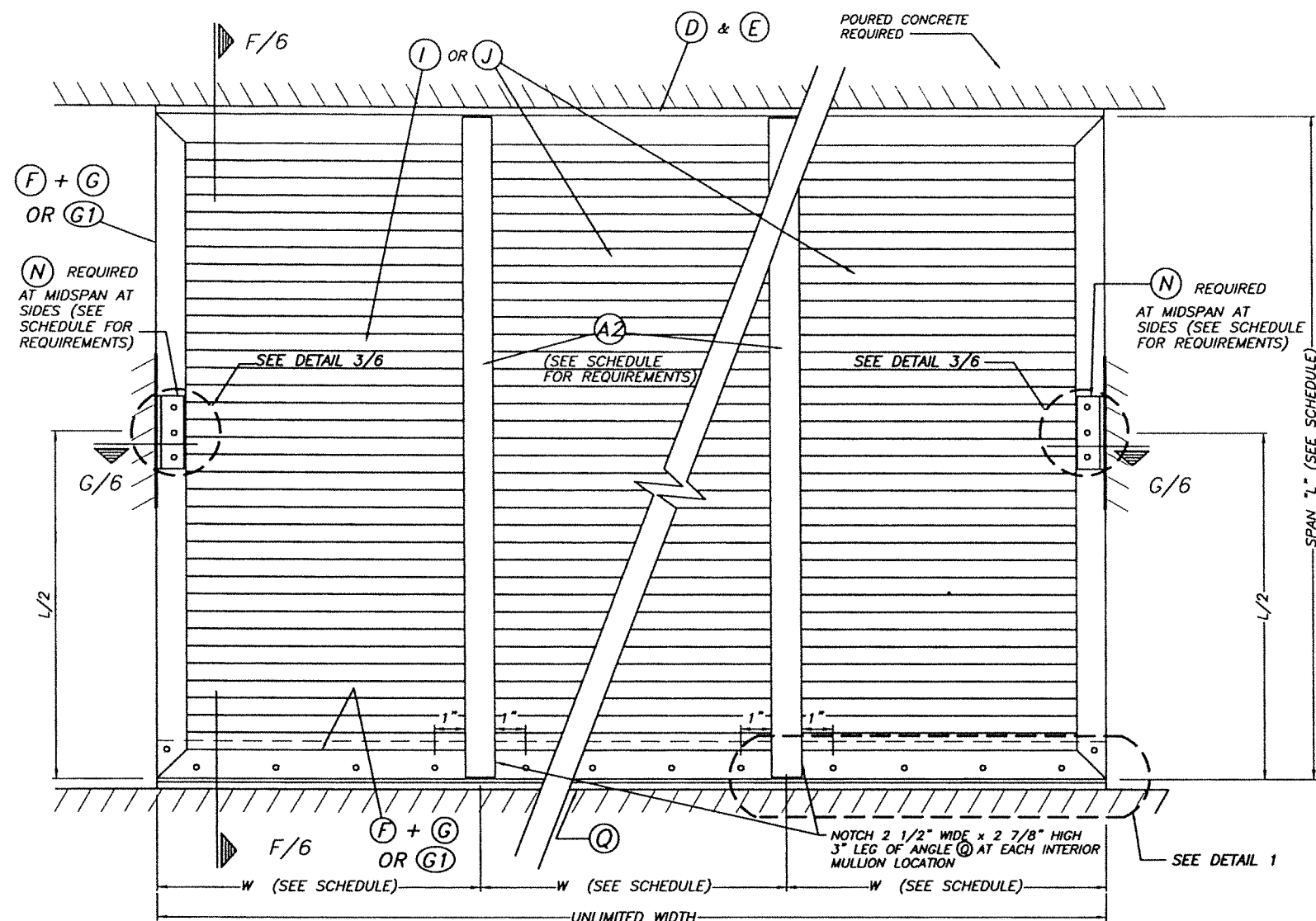
MULTIPLE UNIT
