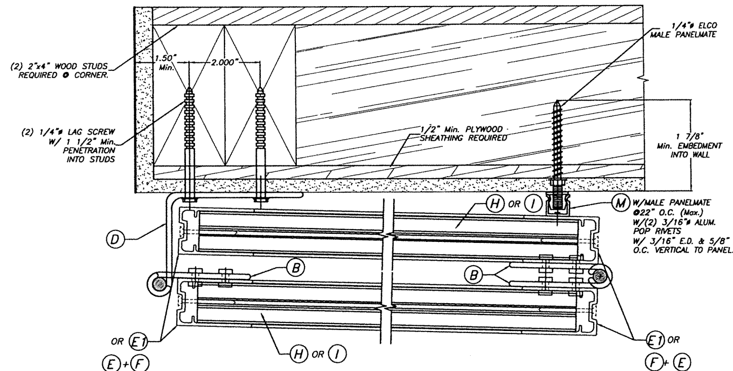
ALTERNATE DETAIL 8A: NON HURRICANE POSITION ONLY (PLAN) SCALE : 3/8" = 1"
