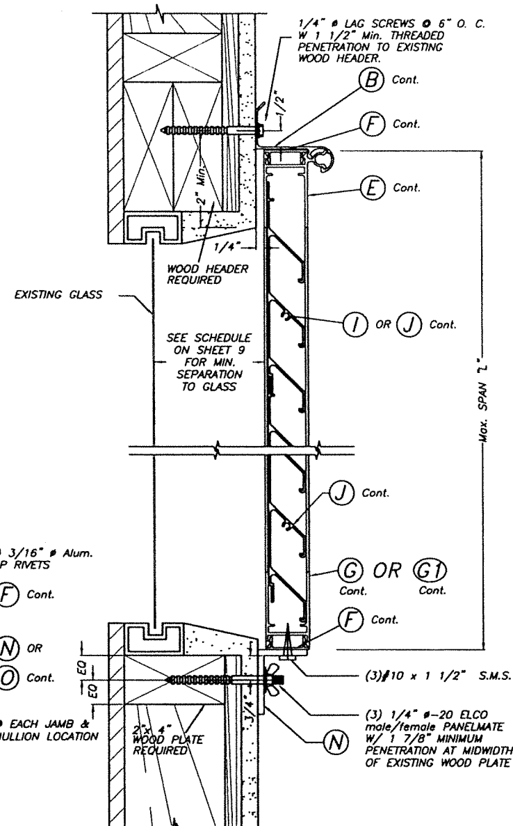
ALTERNATIVE 1 HURRICANE POSITION SCALE: 3/8" = 1"
