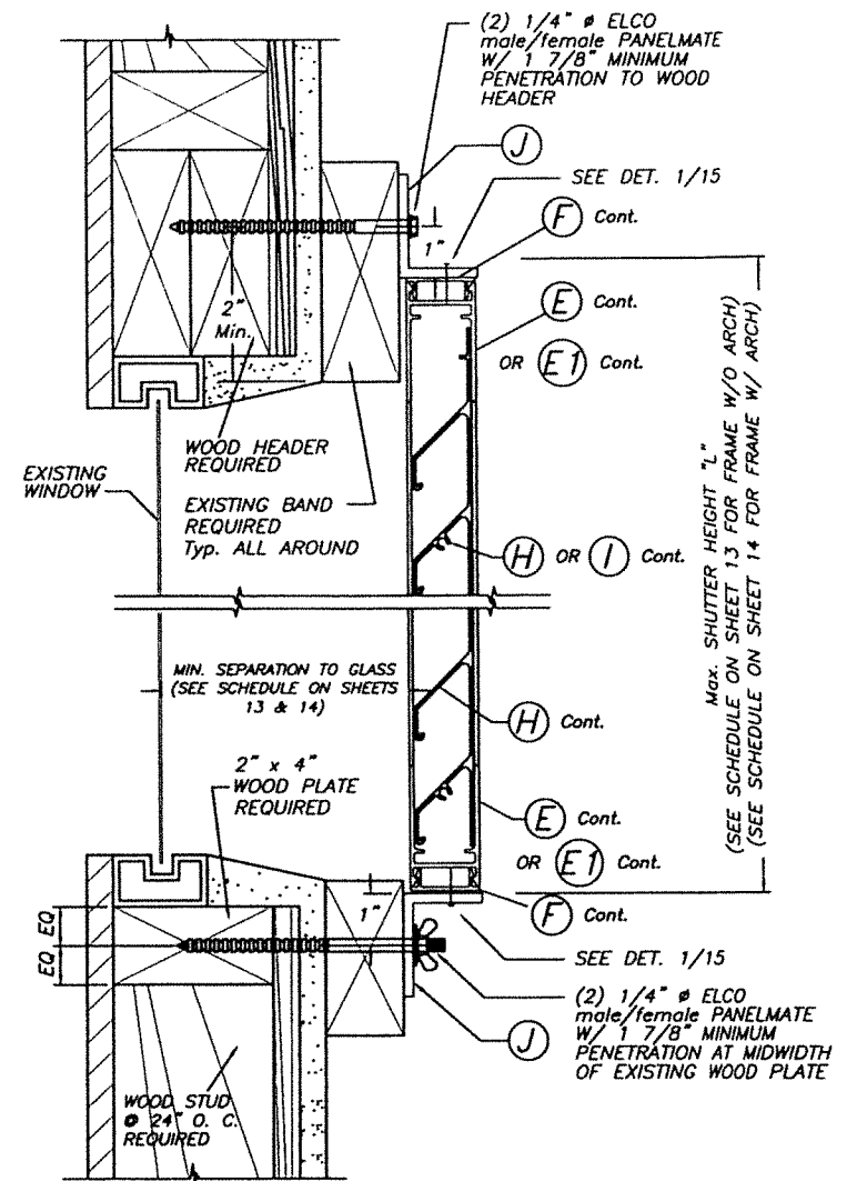
SECTION E' - E' (BUILD-OUT MOUNT) SHUTTER BLADE REVERSELY ORIENTED HURRICANE POSITION SCALE: 1/4" = 1"
