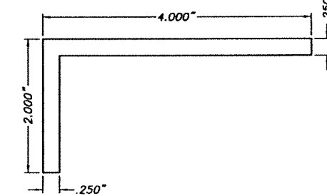
(P) BUILD-OUT SIDE BRACKET 7" LONG SCALE: 1/2" = 1"
