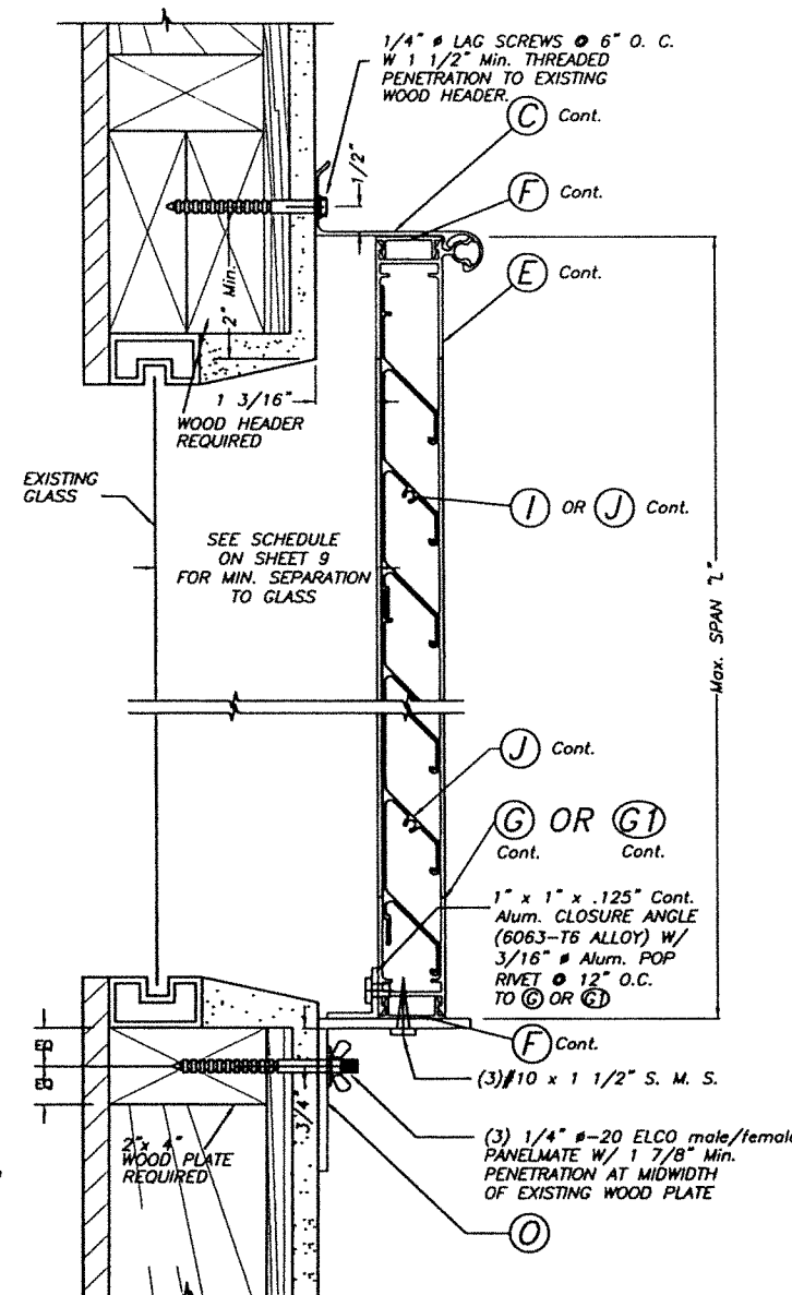
ALTERNATIVE 2 HURRICANE POSITION SCALE: 3/8" = 1"
