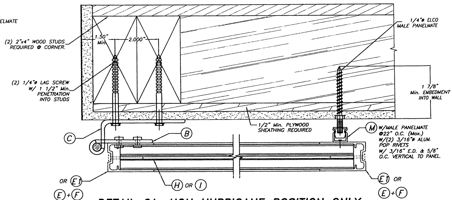
DETAIL 6A: NON HURRICANE POSITION ONLY (PLAN) SCALE : 3/8" = 1"
