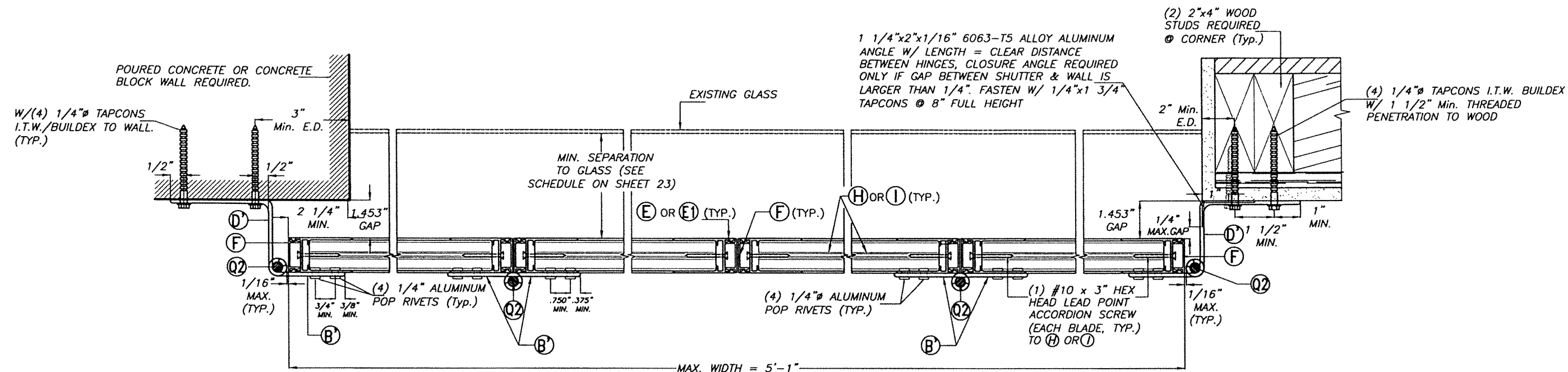
1 SECTION D-D SCALE 1/4"=1"
