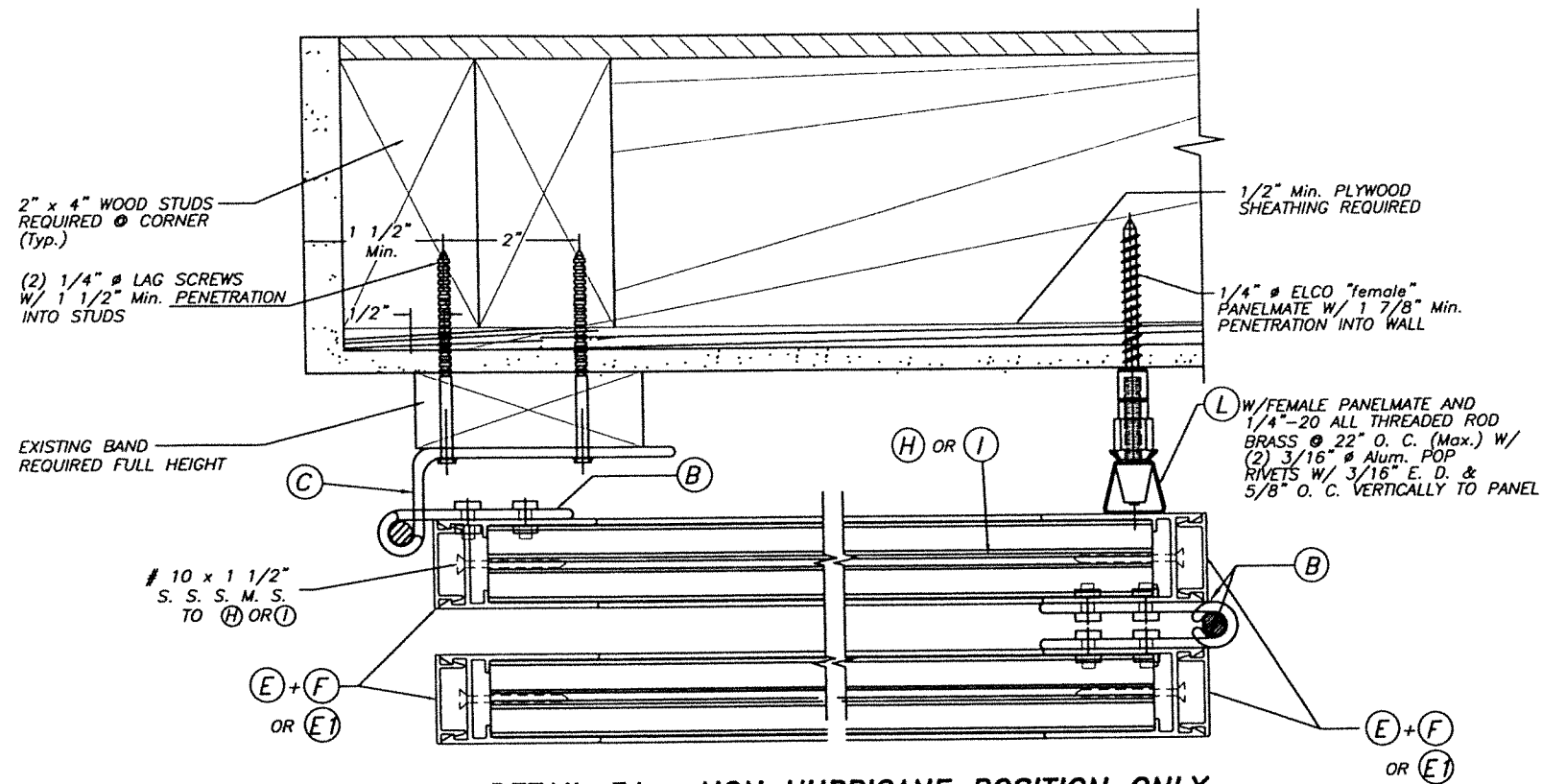
DETAIL 5A : NON HURRICANE POSITION ONLY (PLAN) SCALE : 1/4" = 1"
