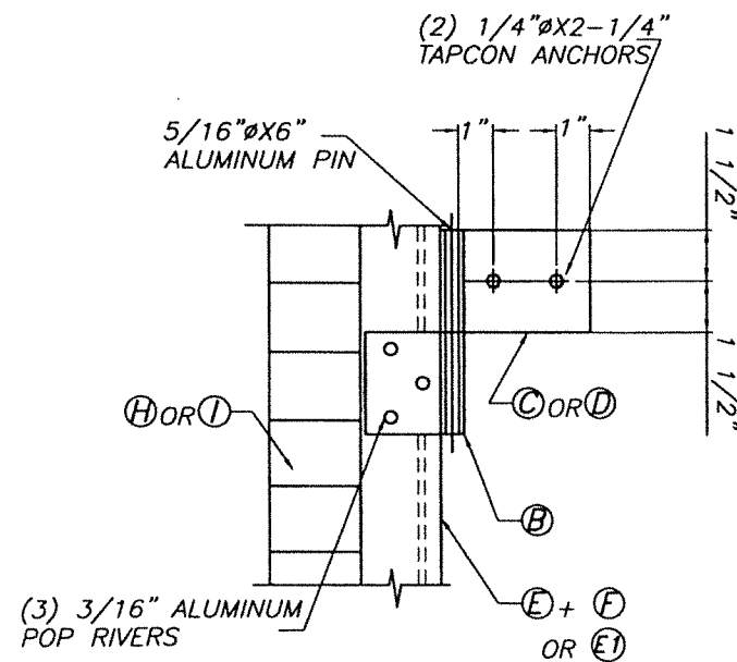
DETAIL 3
