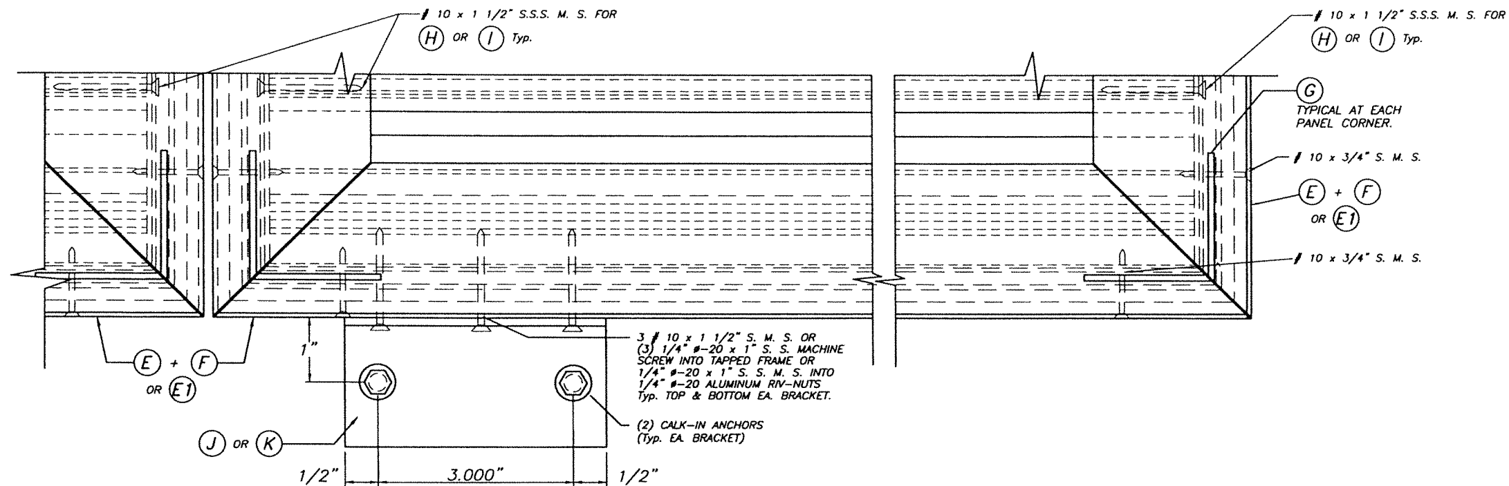
DETAIL 1 SCALE : 1/2" = 1"
